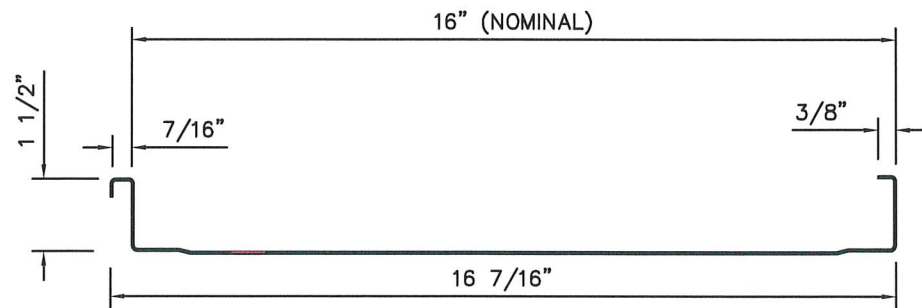
PANEL PROFILE
